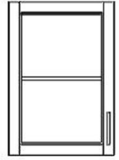
720 & 900 High glass wall unit 720 High - 400,500,600 wide 900 High - 500 wide
